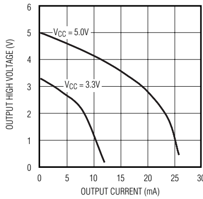
RECEIVER OUTPUT HIGH VOLTAGE vs. OUTPUT CURRENT
